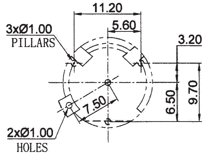
PCB MOUNTING LAYOUT
