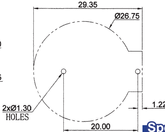
PCB MOUNTING LAYOUT
